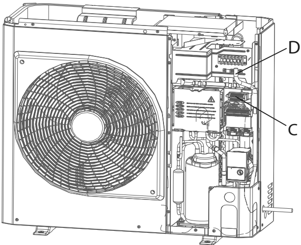
4, 6, 8 kW 1Ph
